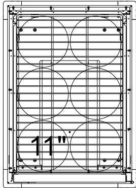
11" Covered Plate Configuration stacked four shelves 4 plates high.
